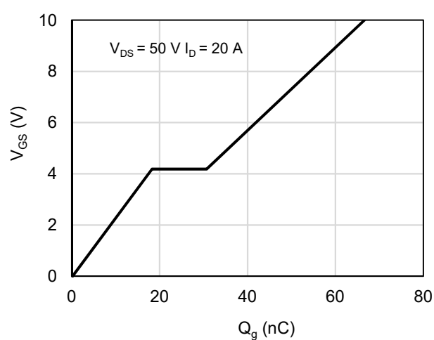
Figure 10: Gate-Charge Characteristics
