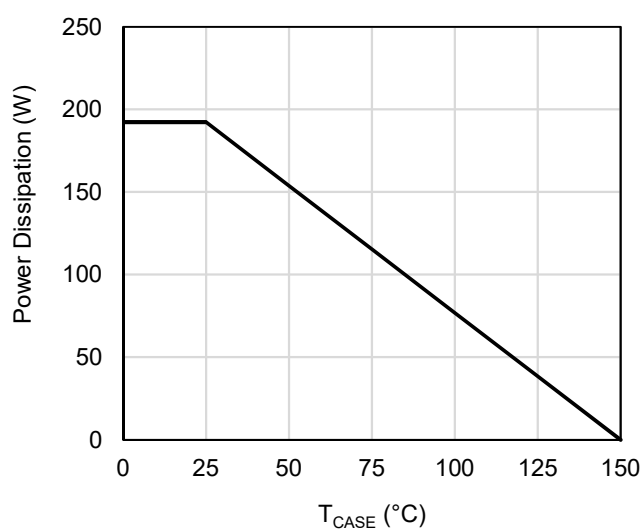
Figure 11: Power De-rating
